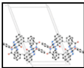
Fig. 2. A partial view of the crystal packing of (I). Dashed lines show C-H... \pi interaction.
